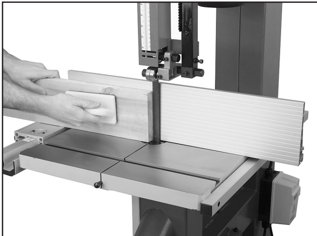
Figure 45. Resawing lumber.
